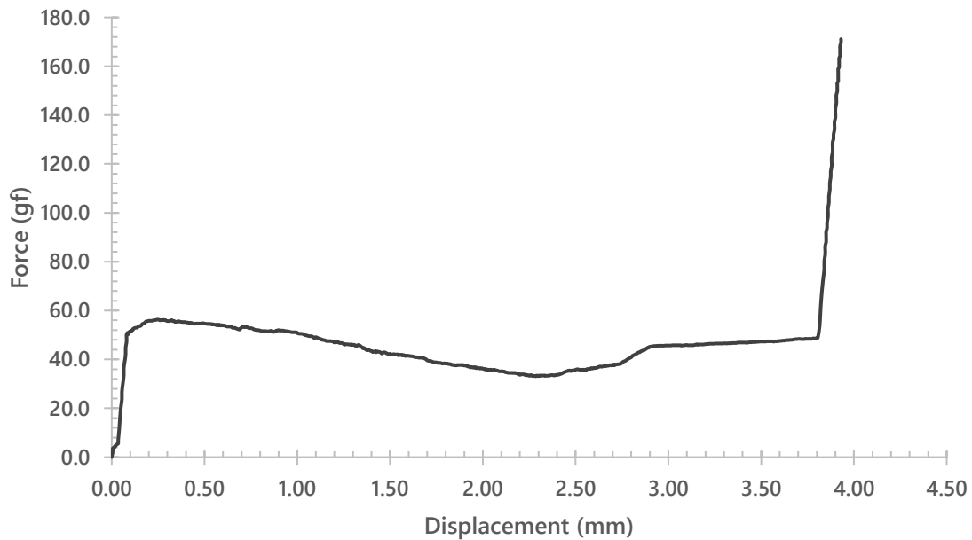
Sillyworks x HMX Waverider V2 (Upstroke)
